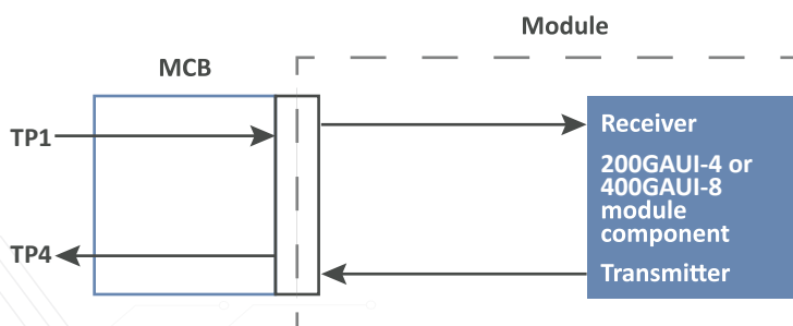
Figure 120E-6—Module 200GAUI-4 or 400GAUI-8 C2M compliance points
